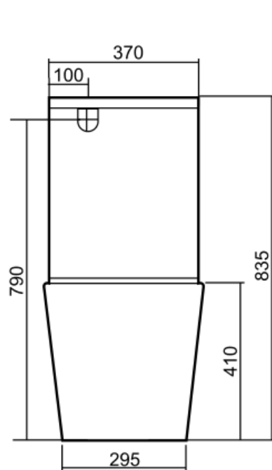
FRONT VIEW
