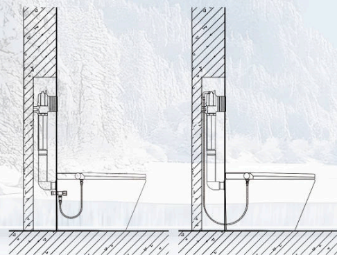
Intalling stop valve
